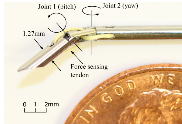
Fig. 1: Steerable needle prototype with orthogonally arranged two hinge joints near tip, composed of a 120 mm long and 1.27 mm outer diameter Nitinol tube and Kevlar connected optical fibers. Multi-lumen polymer tubes guiding tendons are omitted. The rotation range of each joint is designed to be \pm 25^\circ .
